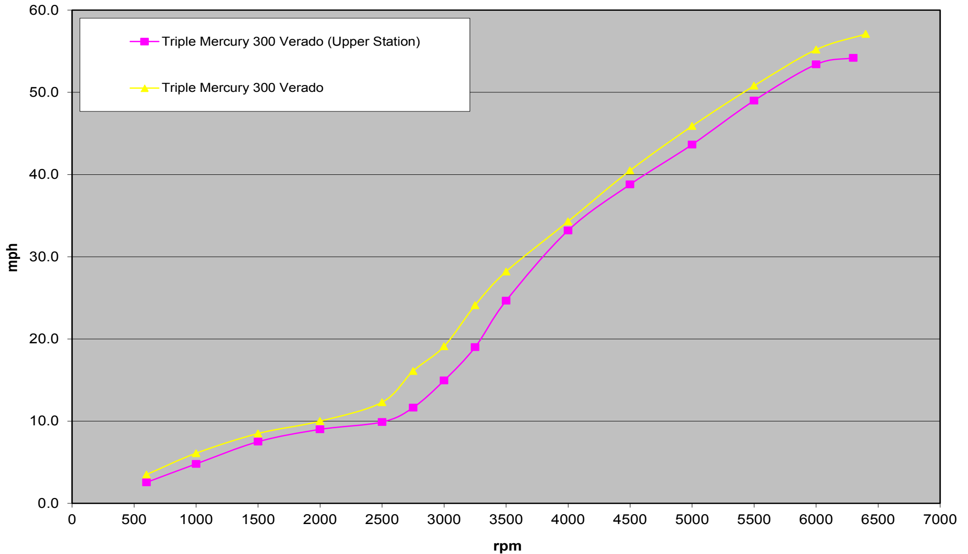
350 Outrage Engine Comparison Graph
